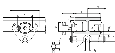
Model HTP/G 500 - 5000 kg
