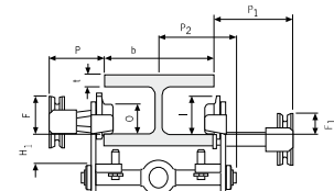
Model HTP/G 500 - 5000 kg, with locking device
